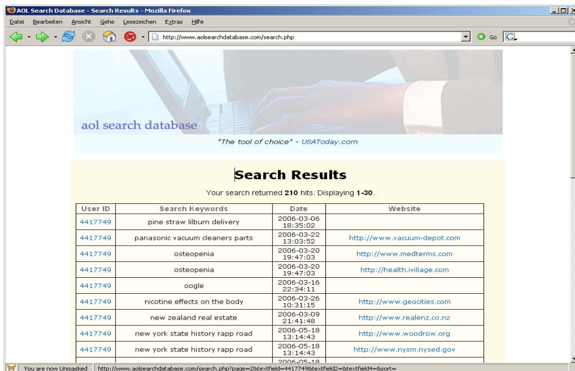
Abbildung 6: Screenshot: AOLsearchdatabase.com
